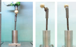
All 3 MP HD 12 mm dia. stems of EndoDur-S survived the ISO test of 5 million cycles with 1200N load.
